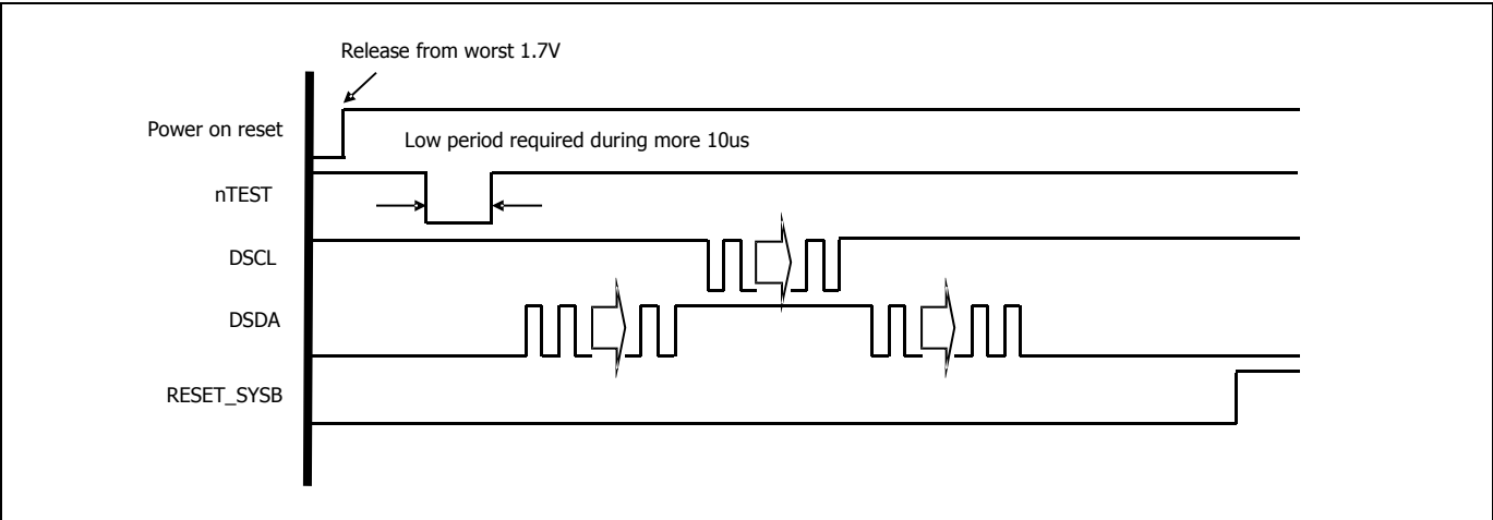
Figure 15.10 ISP mode
