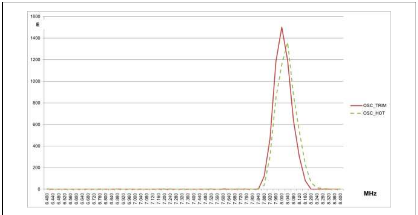
Figure 7.5 8MHz Internal OSC Freq.(OSC_HOT: 85°C)
