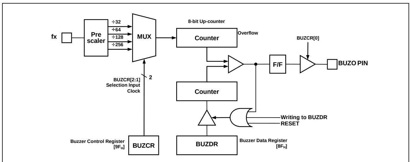
Figure 11.38 Buzzer Driver Block Diagram
