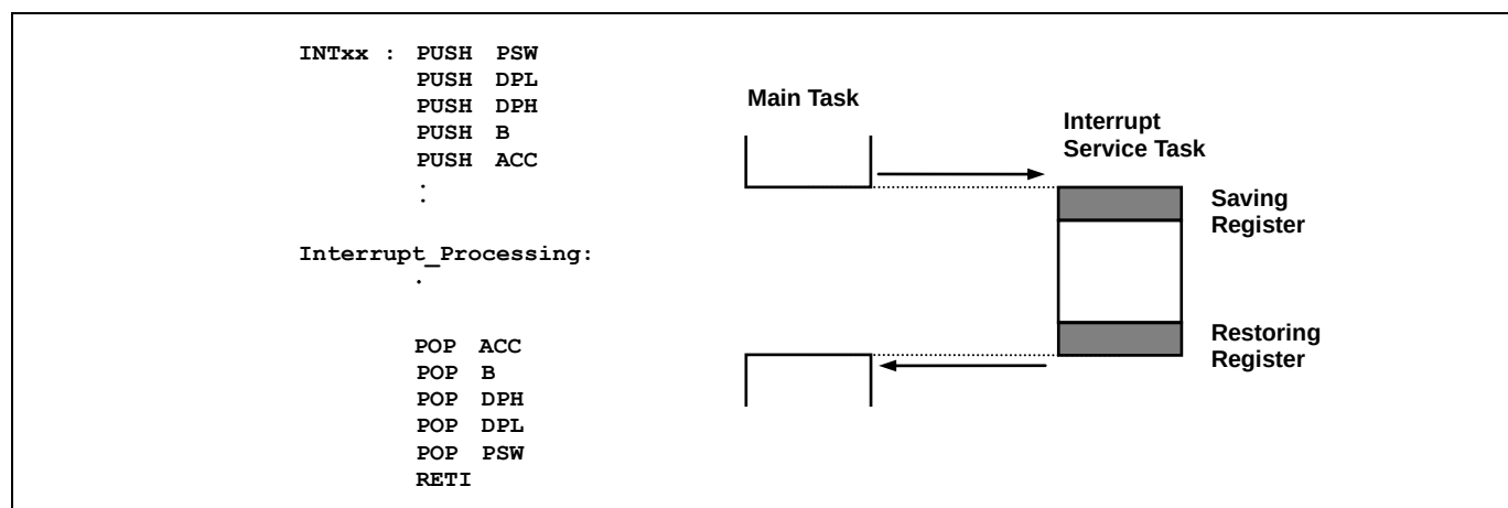
Figure 10.8 Saving/Restore Process Diagram and Sample Source
