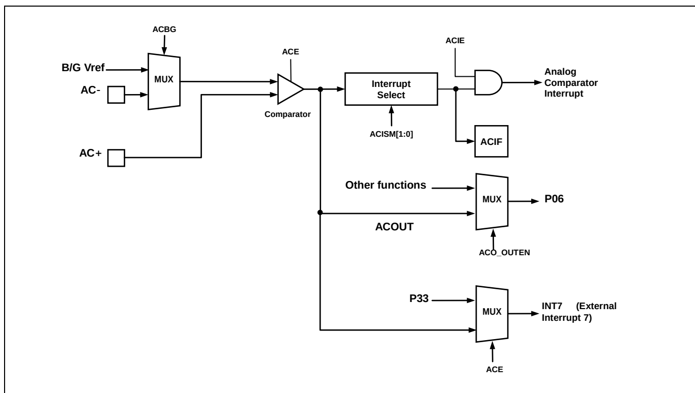
Figure 11.63 Analog Comparator Block Diagram
