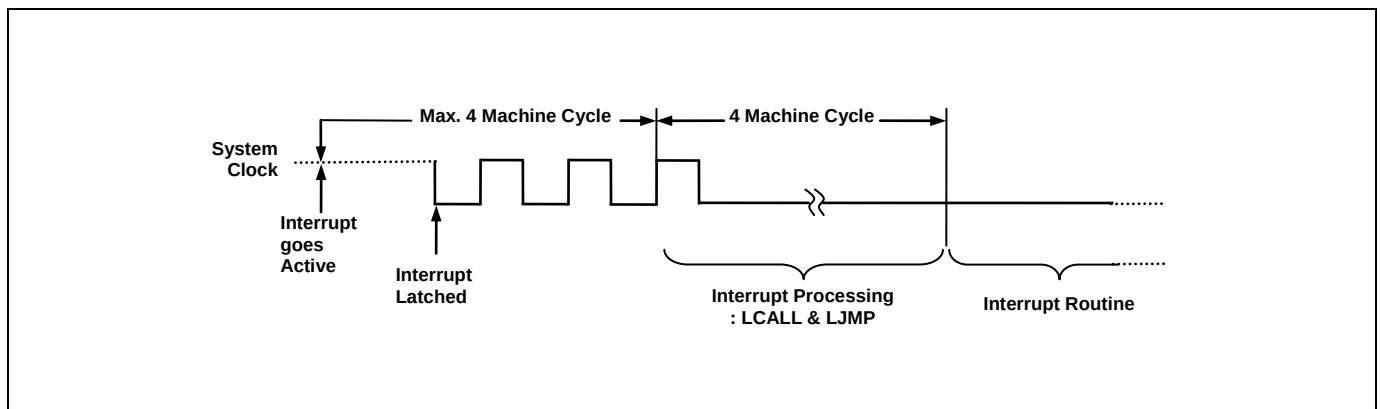
Figure 10.6 Interrupt Response Timing Diagram
