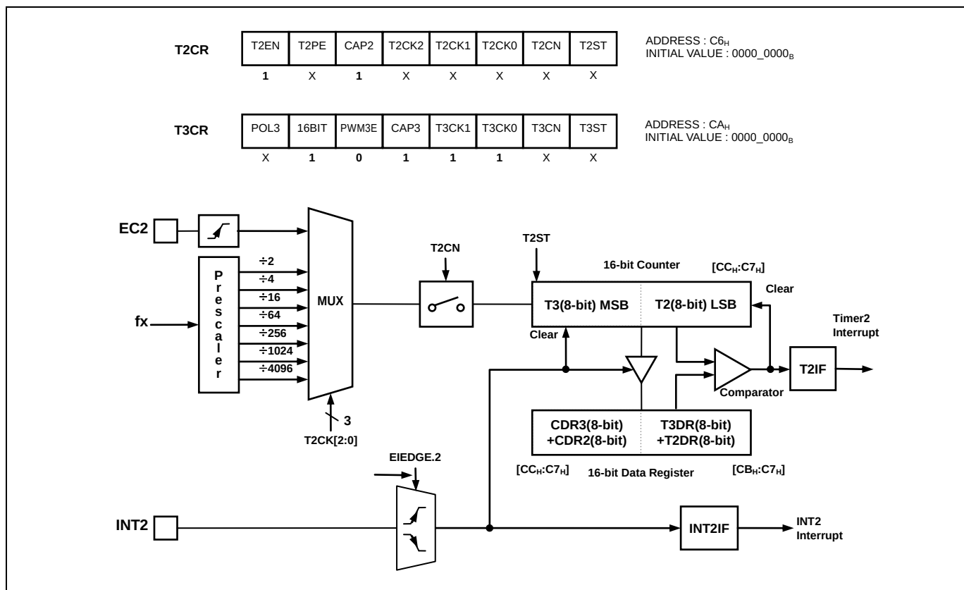
Figure 11.33 16-bit Capture Mode of Timer 2, 3
