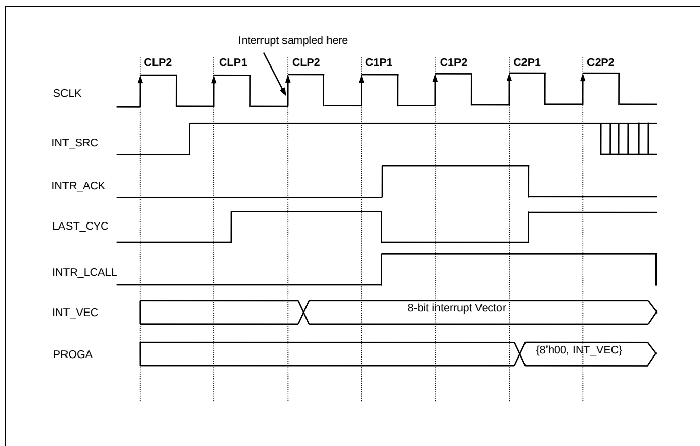
Figure 10.9 Timing Chart of Interrupt Acceptance and Interrupt Return Instruction
