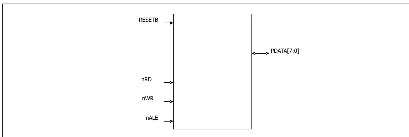
Figure 15.7 Pin diagram for parallel programming
