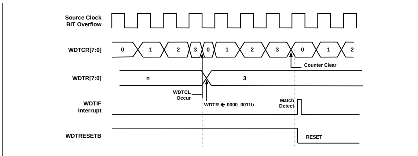
Figure 11.4 WDT Interrupt Timing Waveform
