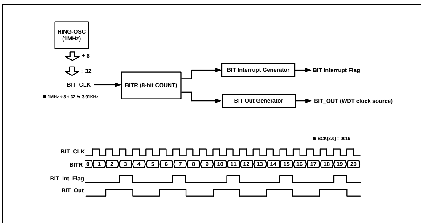
Figure 11.2 Basic Interval Timer Block Diagram
