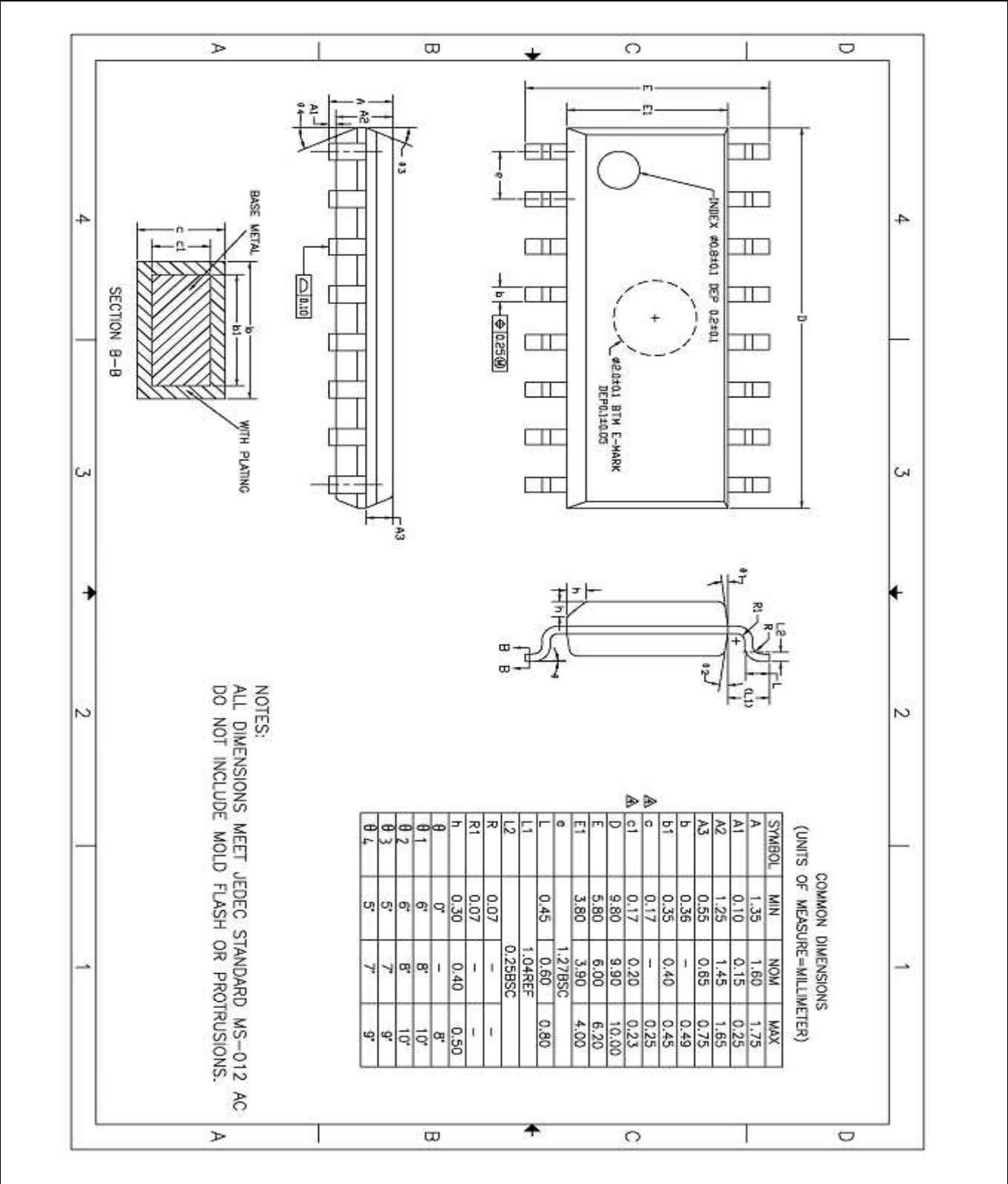
Figure 4.9 16-Pin SOP Package
