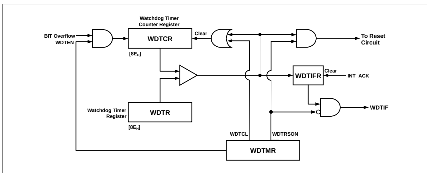
Figure 11.3 WDT Block Diagram
