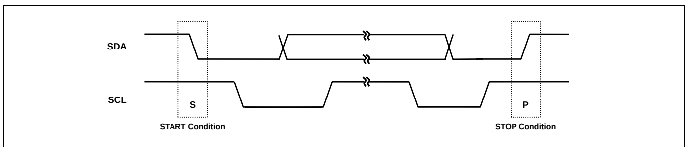
Figure 11.53 START and STOP Condition
