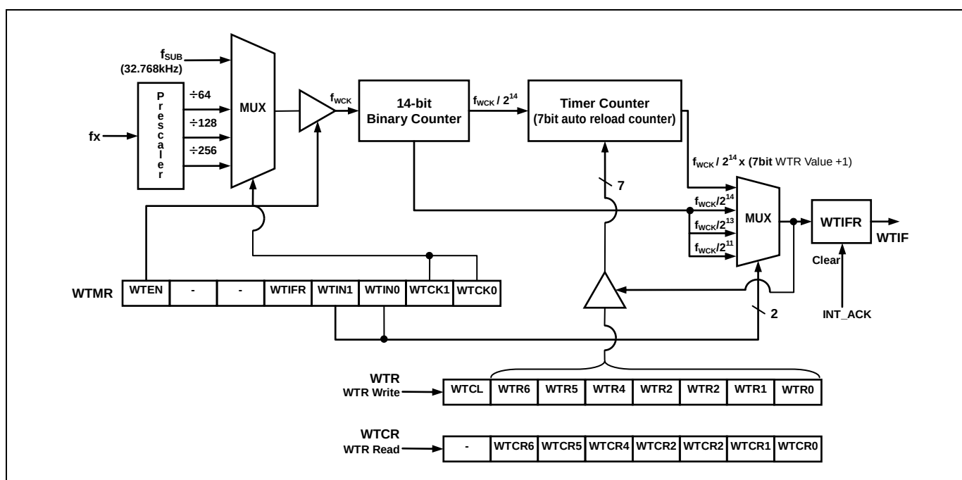
Figure 11.5 Watch Timer Block Diagram
