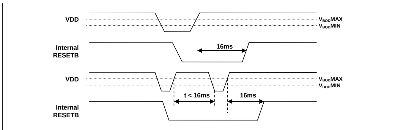
Figure 13.10 Internal Reset at the power fail situation
