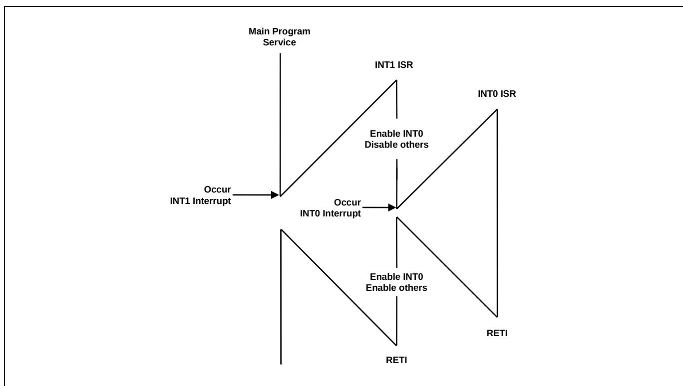
Figure 10.5 Execution of Multi Interrupt
