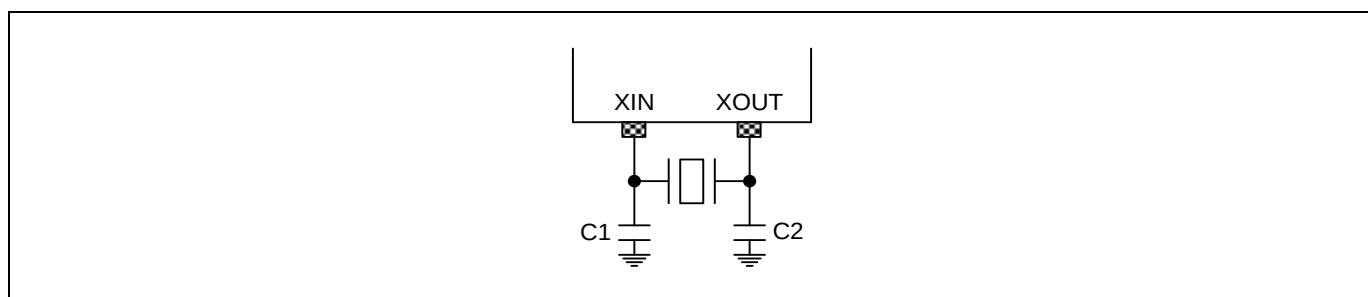
Figure 7.3 Crystal Oscillator
