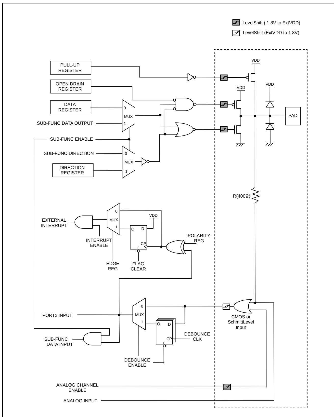
Figure 6.2 External Interrupt I/O Port
