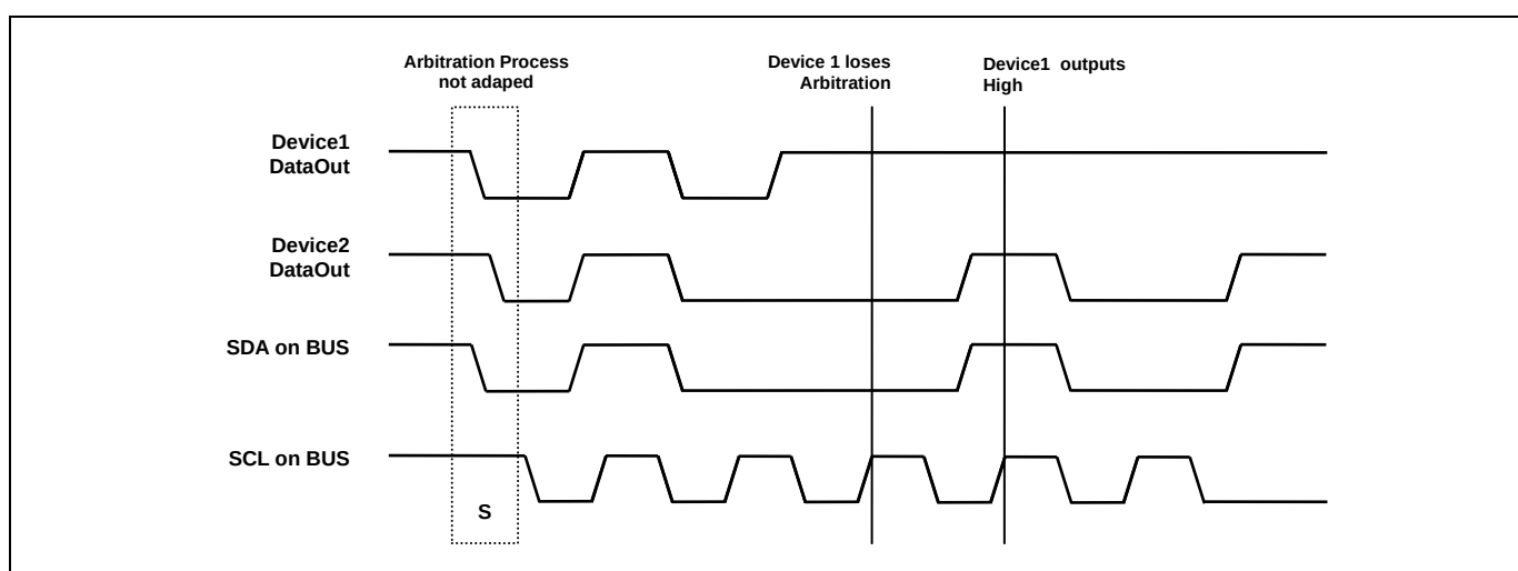
Figure 11.57 Arbitration Procedure of Two Masters
