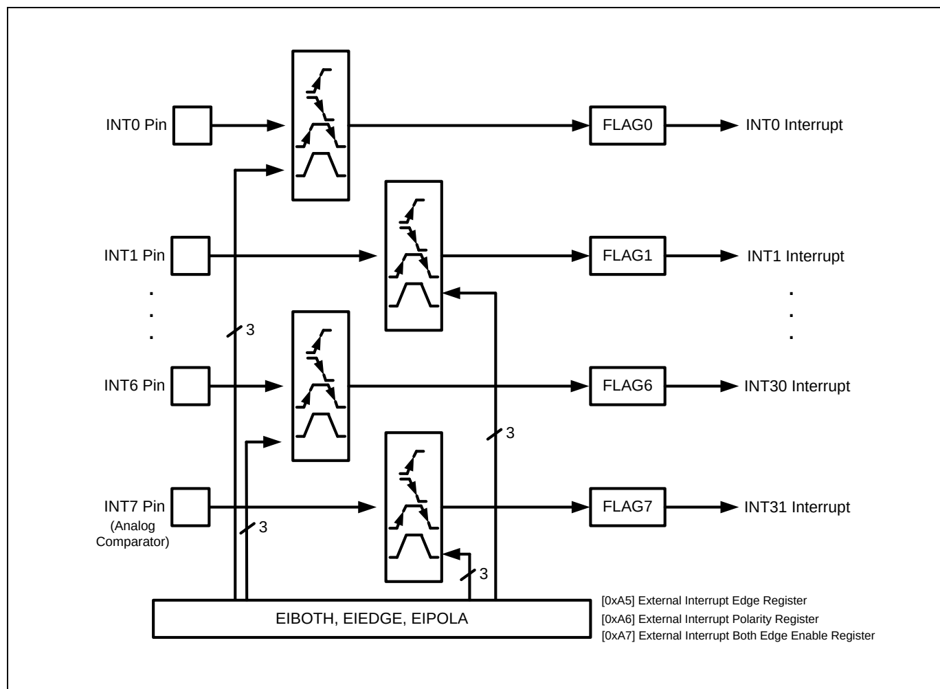
Figure 10.1 External Interrupt Description
