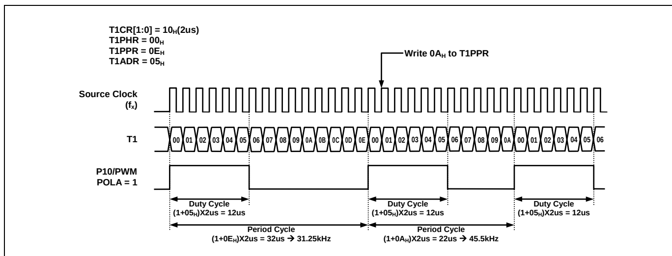
Figure 11.17 Example of Changing the Period in Absolute Duty Cycle at 4Mhz
