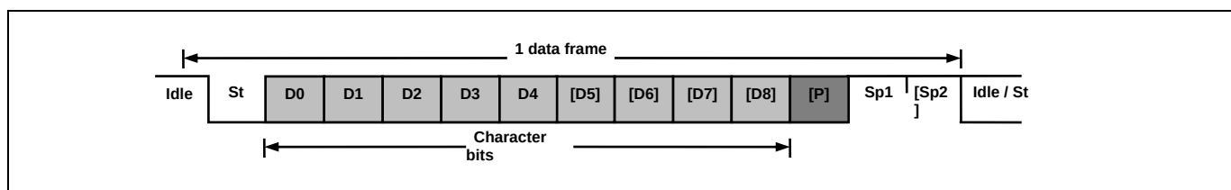
Figure 11.42 frame format
