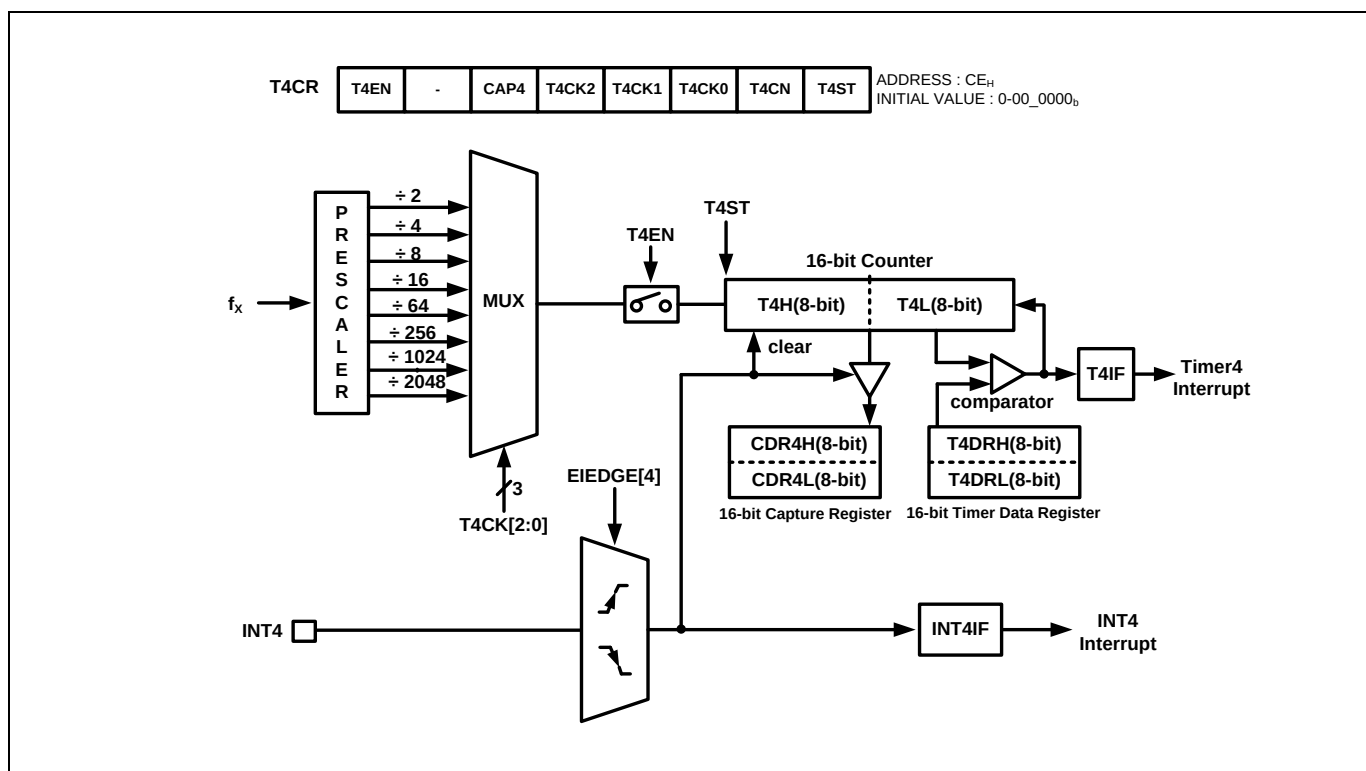
Figure 11.37 Timer4 16-bit Mode Block Diagram
