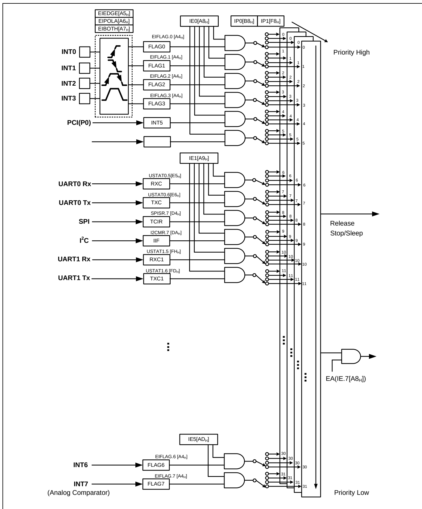
Figure 10.2 Block Diagram of Interrupt
