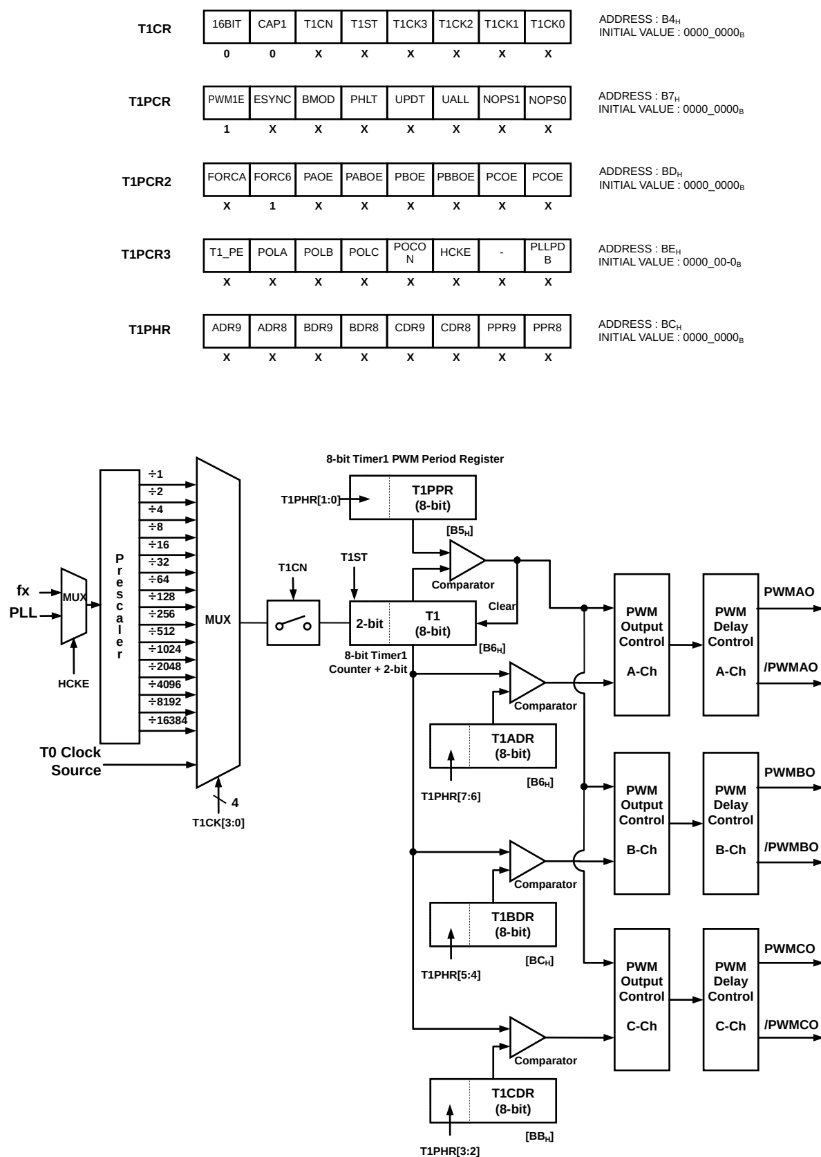
Figure 11.14 PWM Mode (Force 6-ch)
