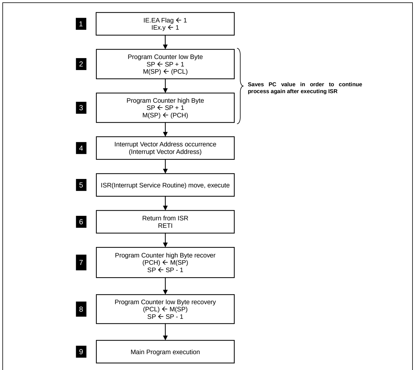
Figure 10.3 Interrupt Sequence Flow
