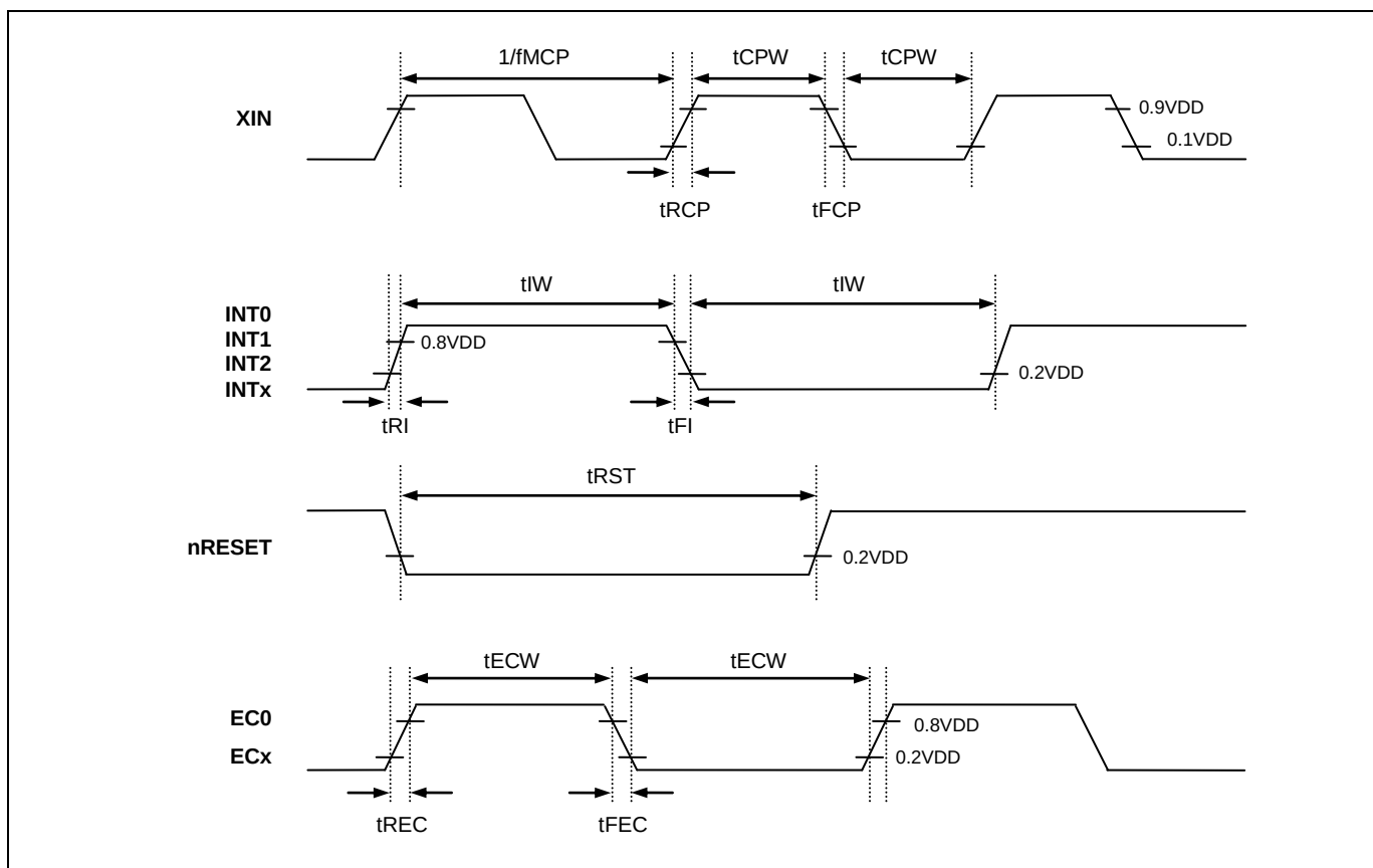
Figure 7.1 AC Timing
