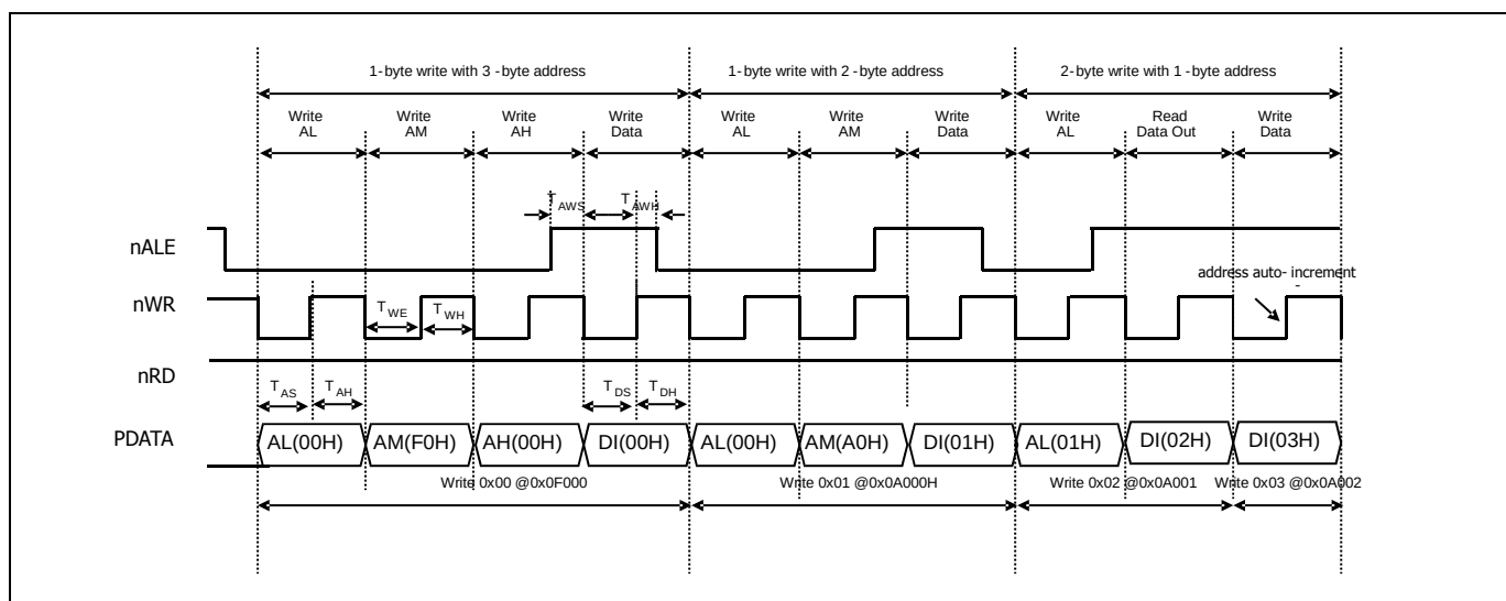
Figure 15.9 Parallel Byte Write Timing of Program Memory
