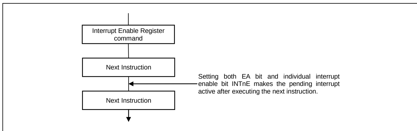
Figure 10.4 Interrupt Enable Register effective Timing
