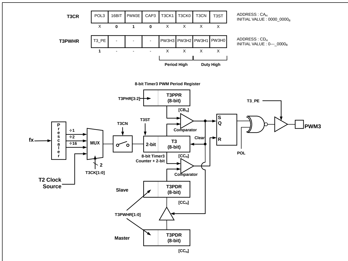
Figure 11.34 PWM Mode
