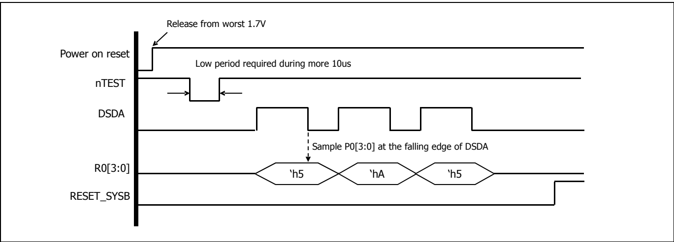
Figure 15.11 Byte-parallel mode
