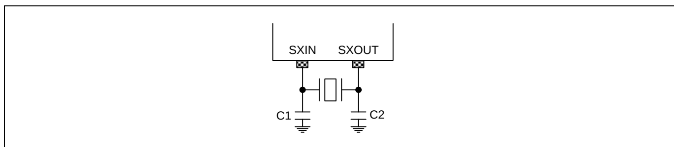
Figure 7.4 Sub-Crystal Oscillator
