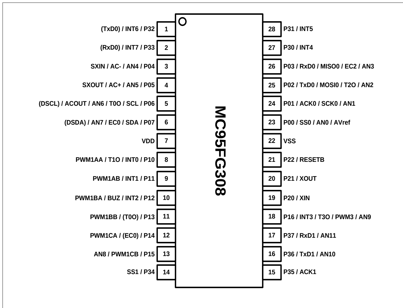
Figure 3.4 MC95FG308 28SOP pin assignment
