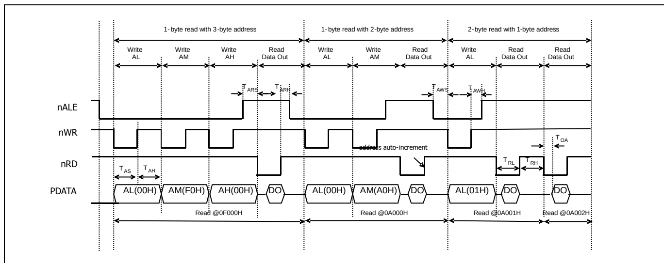
Figure 15.8 Parallel Byte Read Timing of Program Memory
