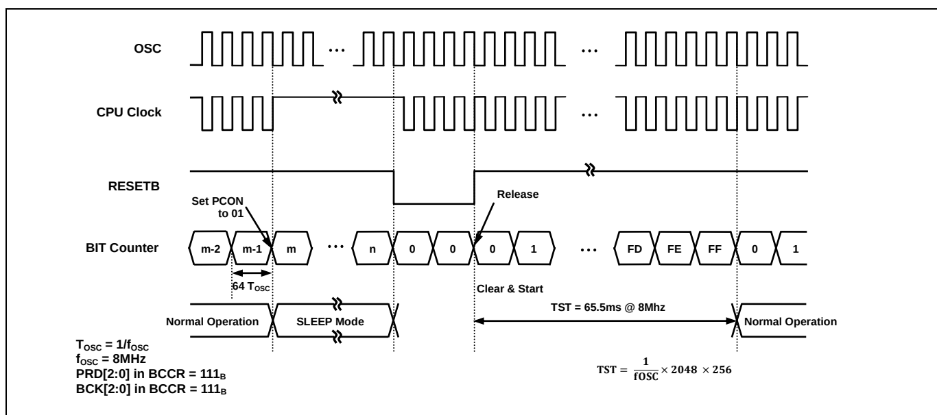
Figure 12.2 IDLE Mode Release Timing by /RESET
