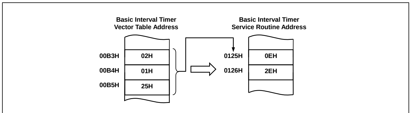
Figure 10.7 Correspondence between Vector Table Address and the Entry Address of ISR
